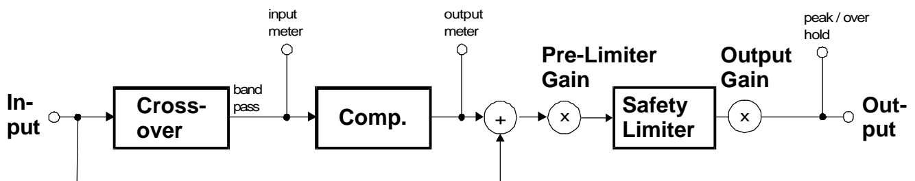
Graphic 11: Parallel band selective compression
