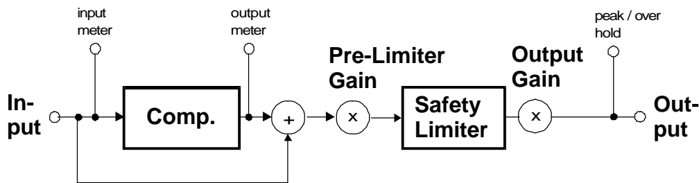
Graphic 10: Parallel full band compression
