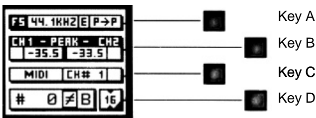
Graph 3: Status Display
