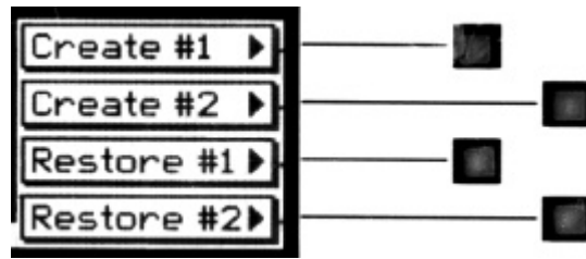
Graph 14: Backup Display
