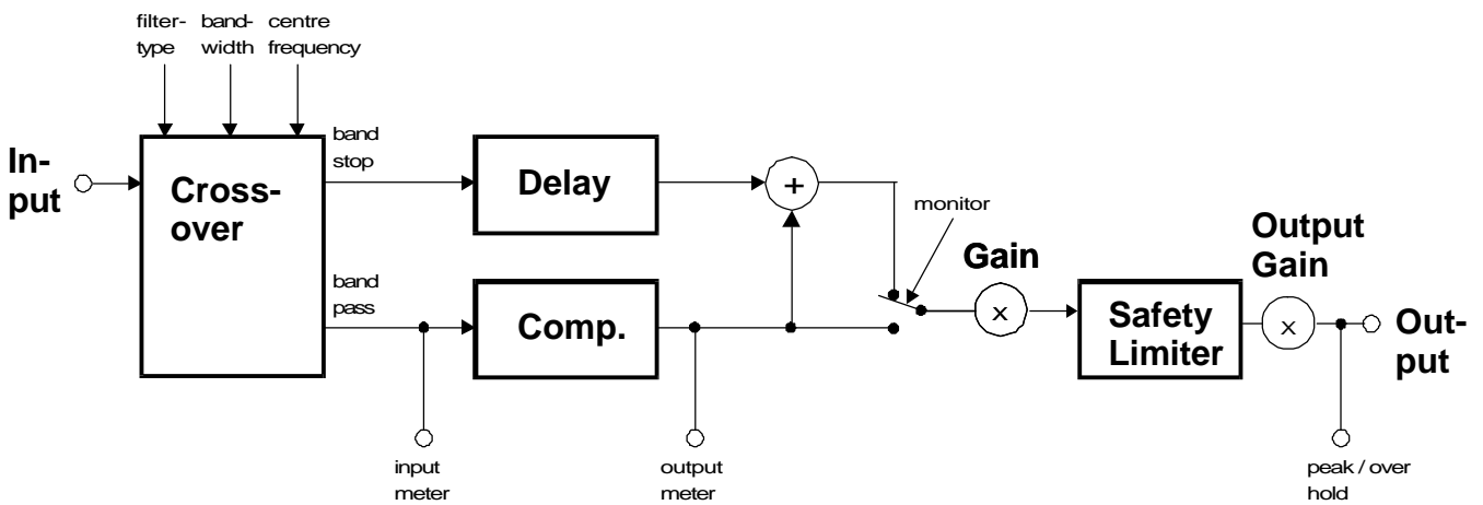
Graphic 8: Band Selective Mode
