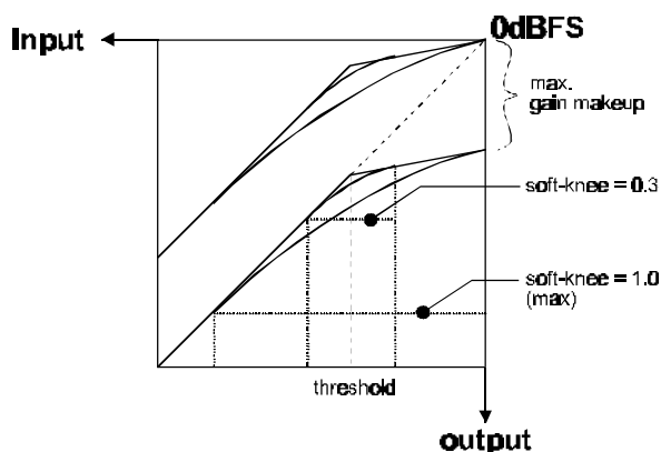
Graphic 7: Transfer Curve Parameters
