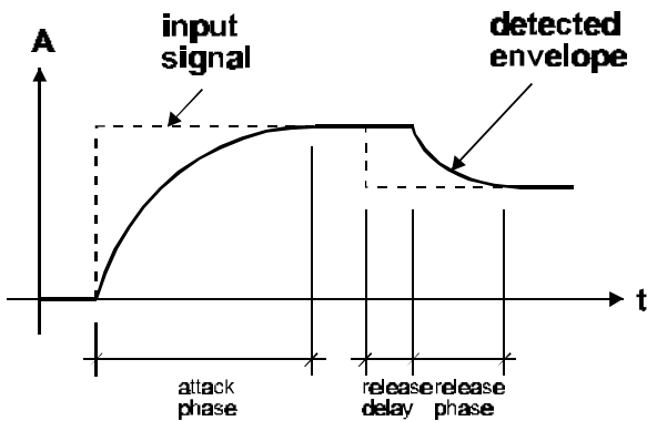
Graphic 6: Envelope Parameters
