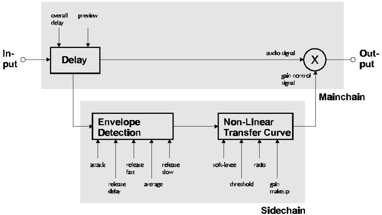
Graphic 5: Compressor schematic
