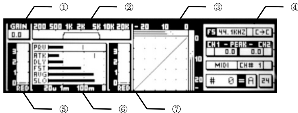
Graphic 2: Display Elements
