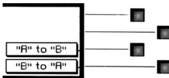
Graph 12: "copy" menu
